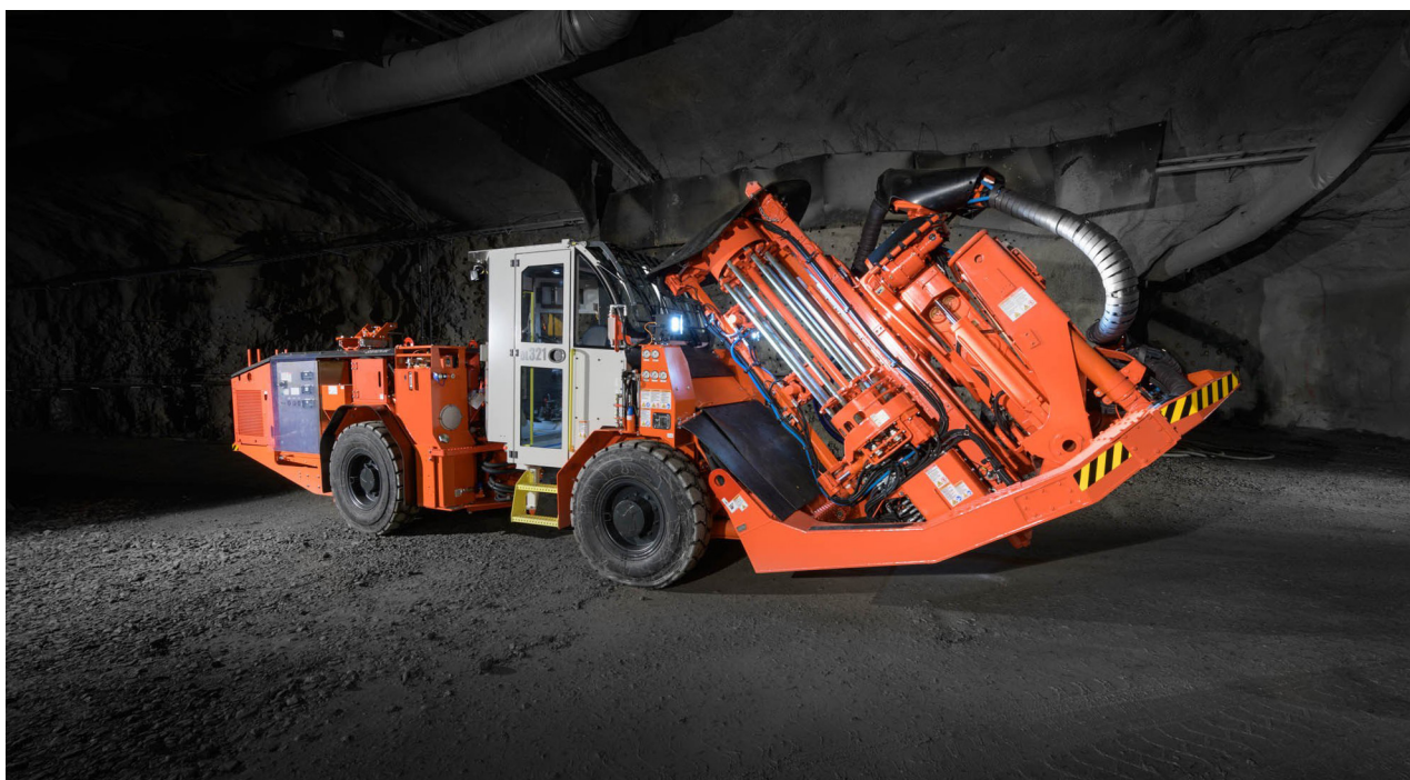
1. DL321 TOP HAMMER - LONGHOLE DRILL
